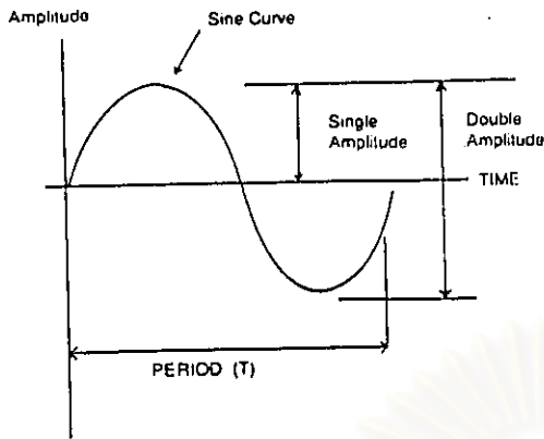
FIG. 4 Definitions Related to Cyclic Loading
