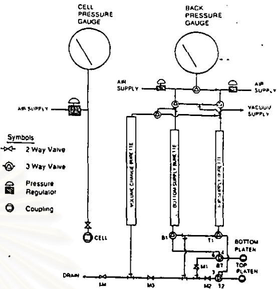
FIG. 8 Pressurizing/Flushing Panel Piping Diagram
