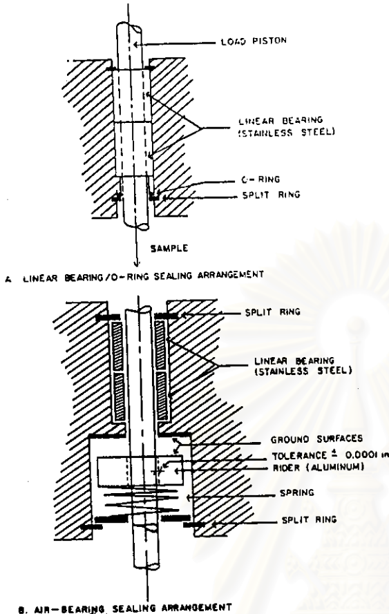
FIG. 10 Typical Cyclic Triaxial Sealing Arrangement
