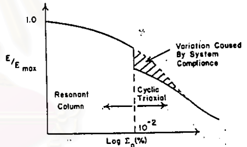
FIG. 12 Variation in Modulus Curves Caused by System Compliance
