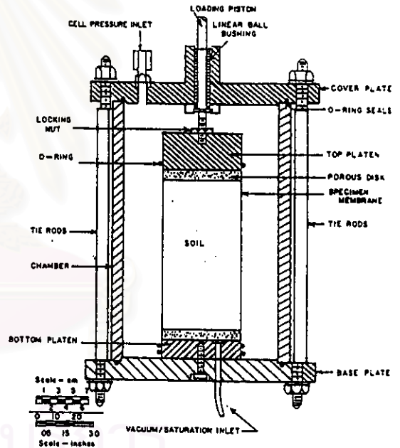
FIG. 3 Typical Cyclic Triaxial Pressure Cell
