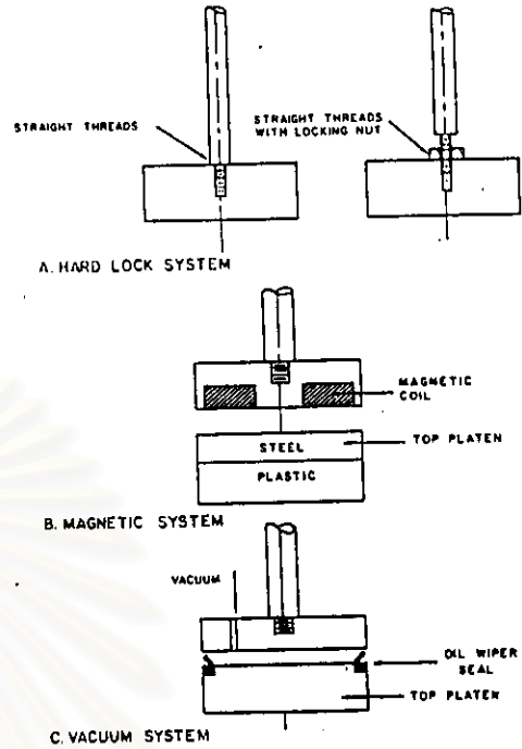
FIG. 6 Top Platen Connections
