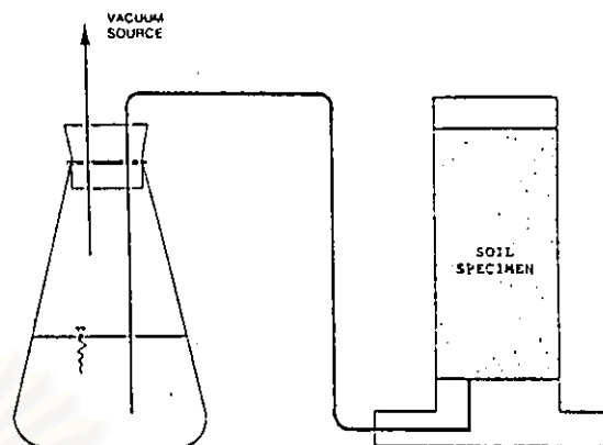
FIG. 9 Method of Applying Vacuum To Soil Samples
