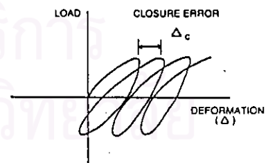
FIG. 13 Definition of Closure Error
