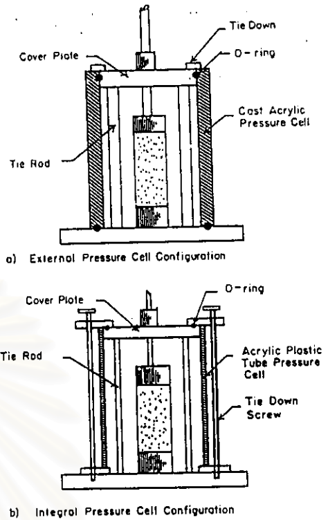
FIG. 11 Typical Design Variations in Aligned Triaxial Pressure Cells
