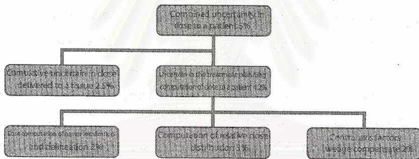
Figure 14. Dosimetric uncertainties in the process of radiation therapy. The uncertainties represent approximately 95 % of confidence level.
