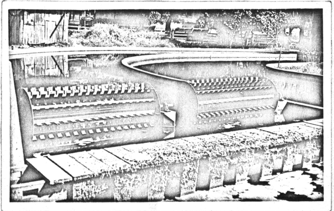
SHOWS THE CAGE ROTOR AT TAK HOSPITAL WASTE TREATMENT PLANT
