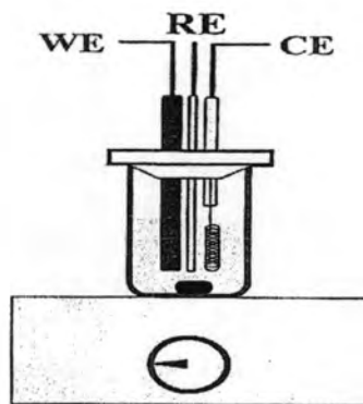
Figure 3.2 Electrochemical cell for SWASV.
