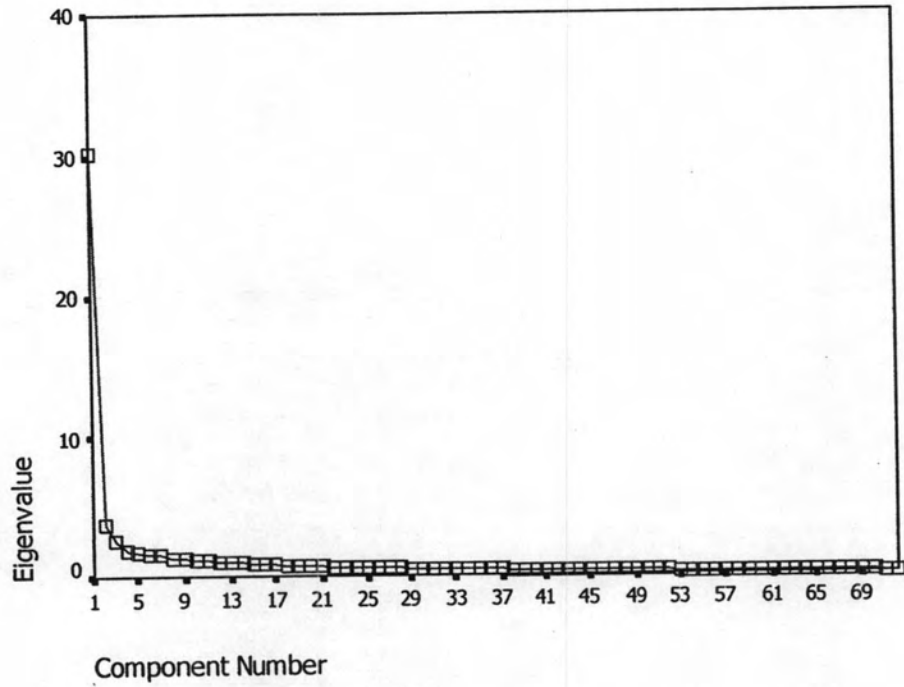
Scree Plot
