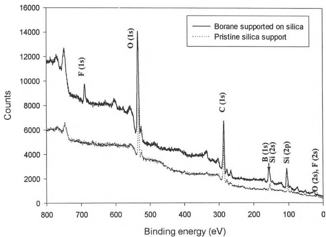
Figure 4.2 XPS survey spectra of borane-supported indicated elements on silica surface (BB supported borane from table 4.1).
