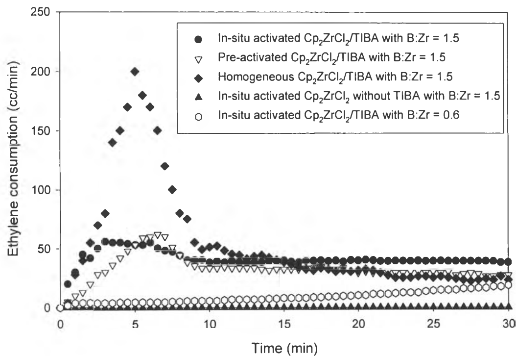
Figure 4.4 Kinetic profiles of ethylene consumption during polymerization with different metallocene system: [\text{Zr}] = 1.6 \mu\text{mol} , \text{Al:Zr} = 400 (in case of desire), \text{B:Zr} = 1.5:1 , T_p = 40^\circ\text{C} , ethylene = 20 psig.
