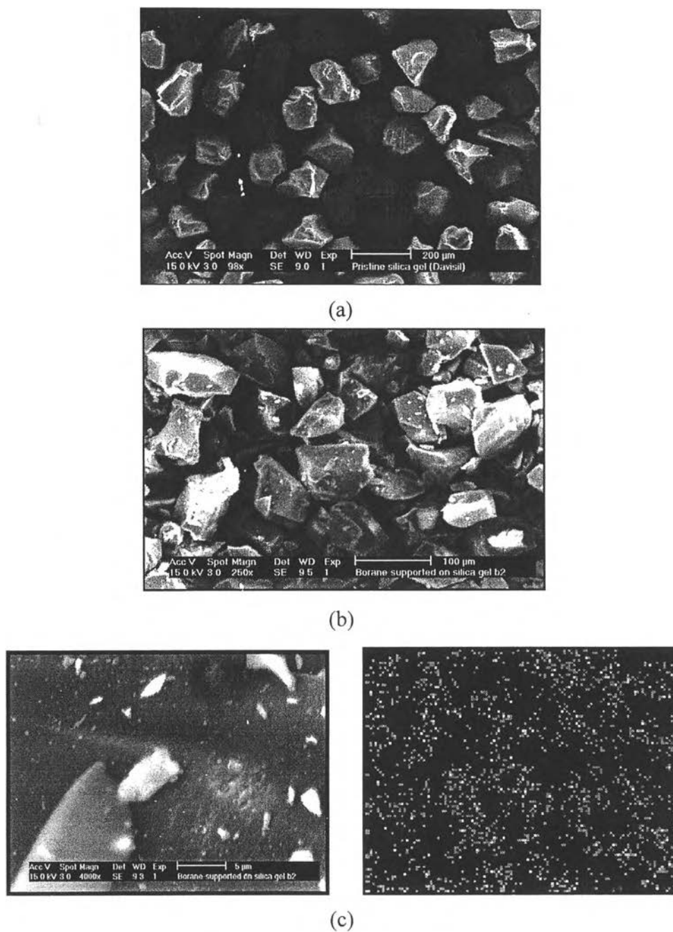
Figure 4.3 SEM micrographs of (a) pristine silica support, (b) borane-supported catalyst, and (c) An enlarged region of silica surface (left), Fluorine-mapping (F-K) of borane on the same silica surface (right).
