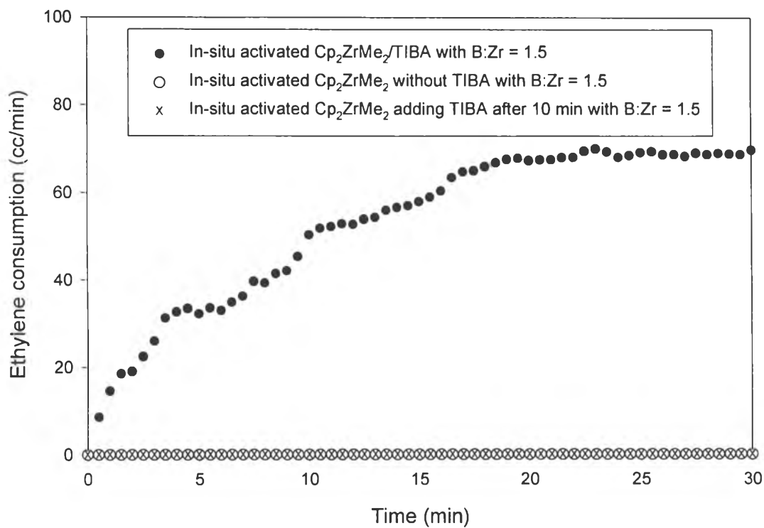
Figure 4.5 Kinetic profiles of ethylene consumption during polymerization with in-situ activated \text{Cp}_2\text{Zr}(\text{CH}_3)_2 : [\text{Zr}] = 19.1 \mu\text{mol} , Al:Zr = 50 (in case of desire), B:Zr = 1.5:1, T_p = 40^\circ\text{C} , ethylene = 20 psig.
