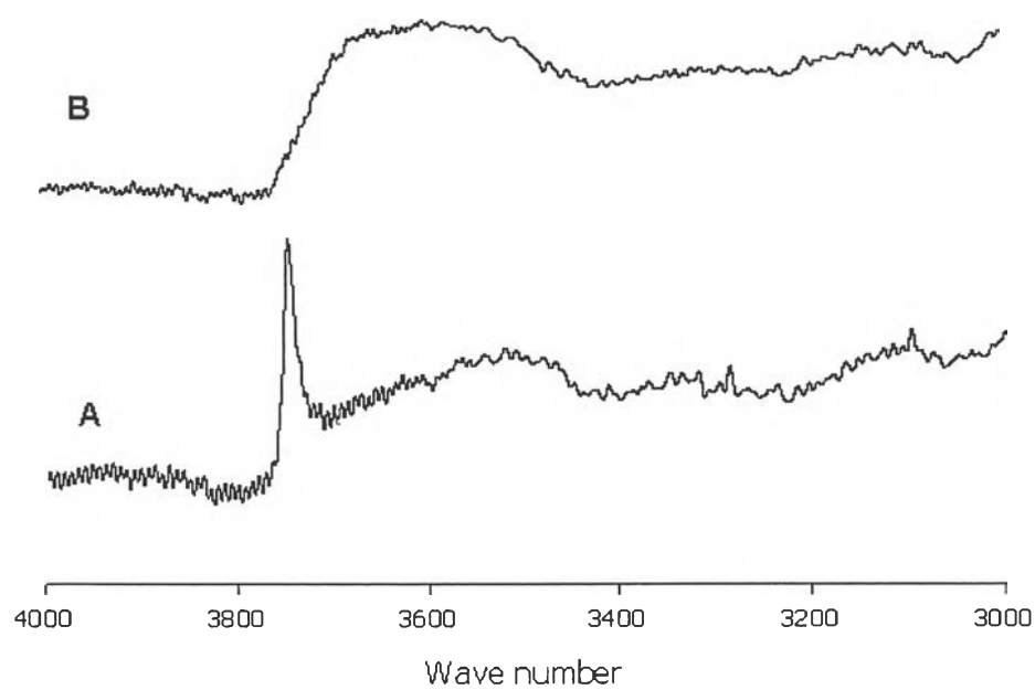
Figure 4.1 FTIR spectra of borane-supported on silica, (A) Silica support at temperature 500 °C calcination, (B) SiO 2 -B(C 6 F 5 ) 3 catalyst. The sharp peak is due to isolated silanol group.
