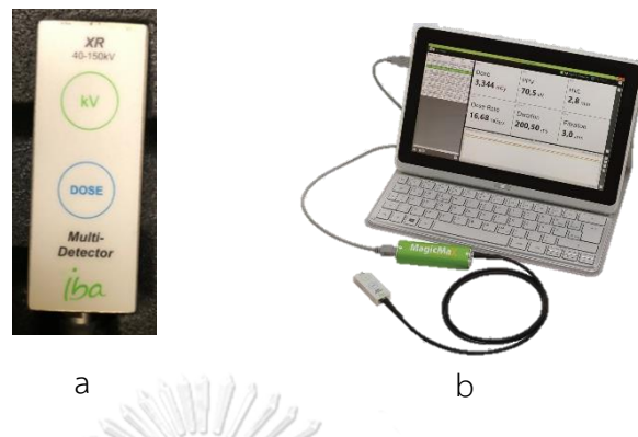
Figure 3. 3 Reference dosimeter, a. Solid state dosimeter (XR multi-detector), b.
