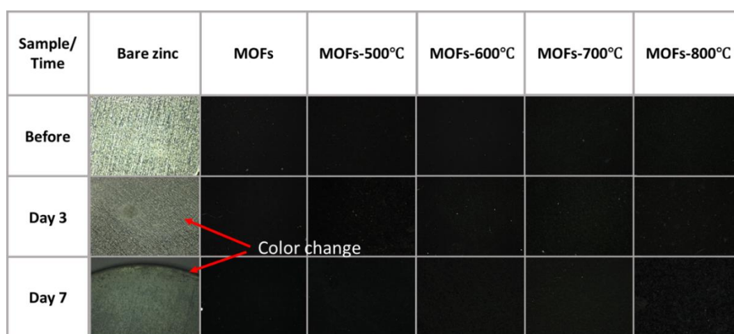
Figure 4.7 Photographs of bare Zn and coated Zn soaked in a 2 M ZnSO 4 electrolyte.
