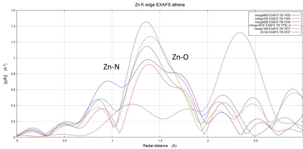
4.5 XAS (Zn K-edge EXAFS) pattern of Zn-BTC-Imidazole (MOFs, MOFs-500°C, MOFs-600°C, MOFs-700°C, and MOFs-800°C)
