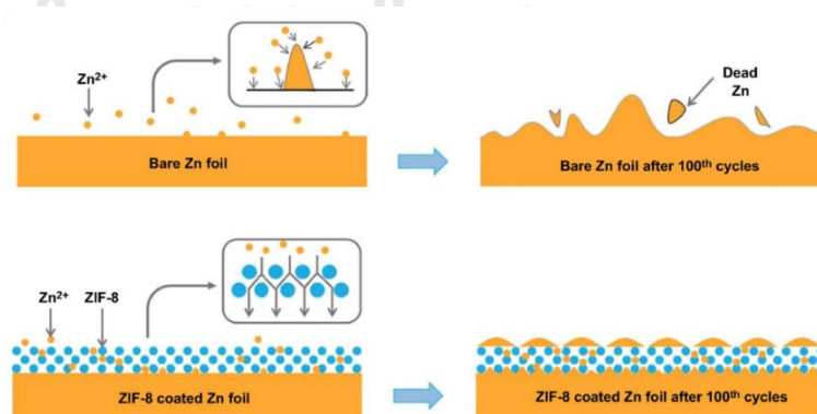
Figure 2.6 Schematic illustration for the morphology of the bare Zn and ZIF-8@Zn electrodes during zinc stripping/plating. [13]
