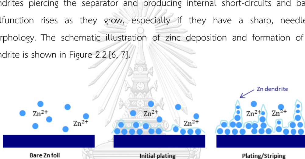
Figure 2.2 Schematic illustration of zinc deposition on bare Zn and the formation of zinc dendrite.
