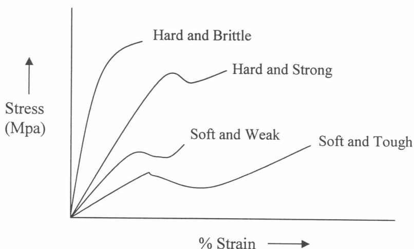
Figure 8 Characteristic of polymer properties in stress-strain curves
