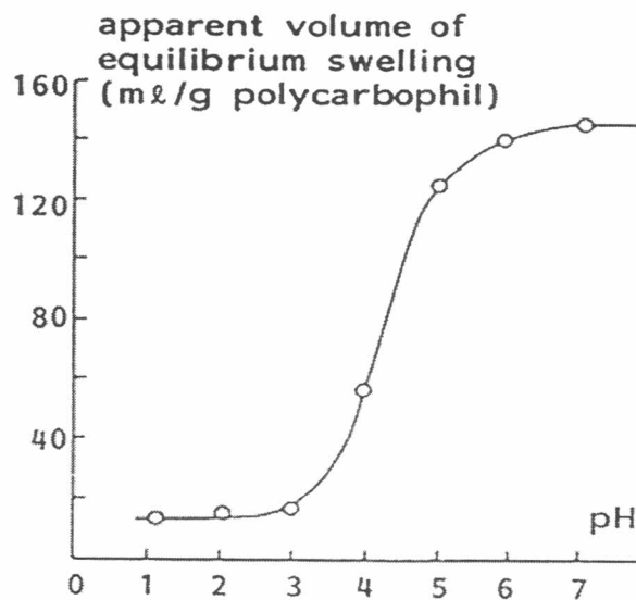
Figure 5 Apparent volume of equilibrium swelling of polycarbophil at various pH (Park and Robinson, 1985)
