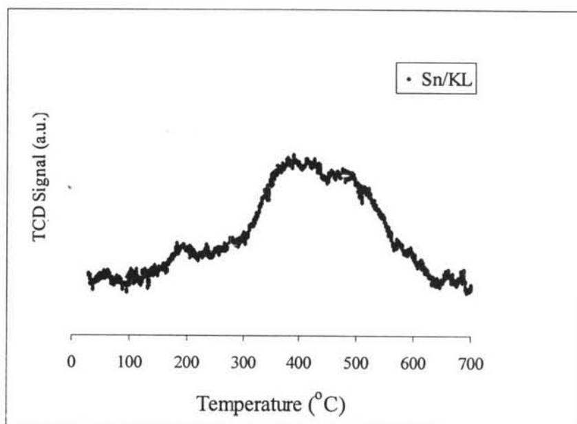
Figure A1 TPR profile for the Sn/KL catalyst.
