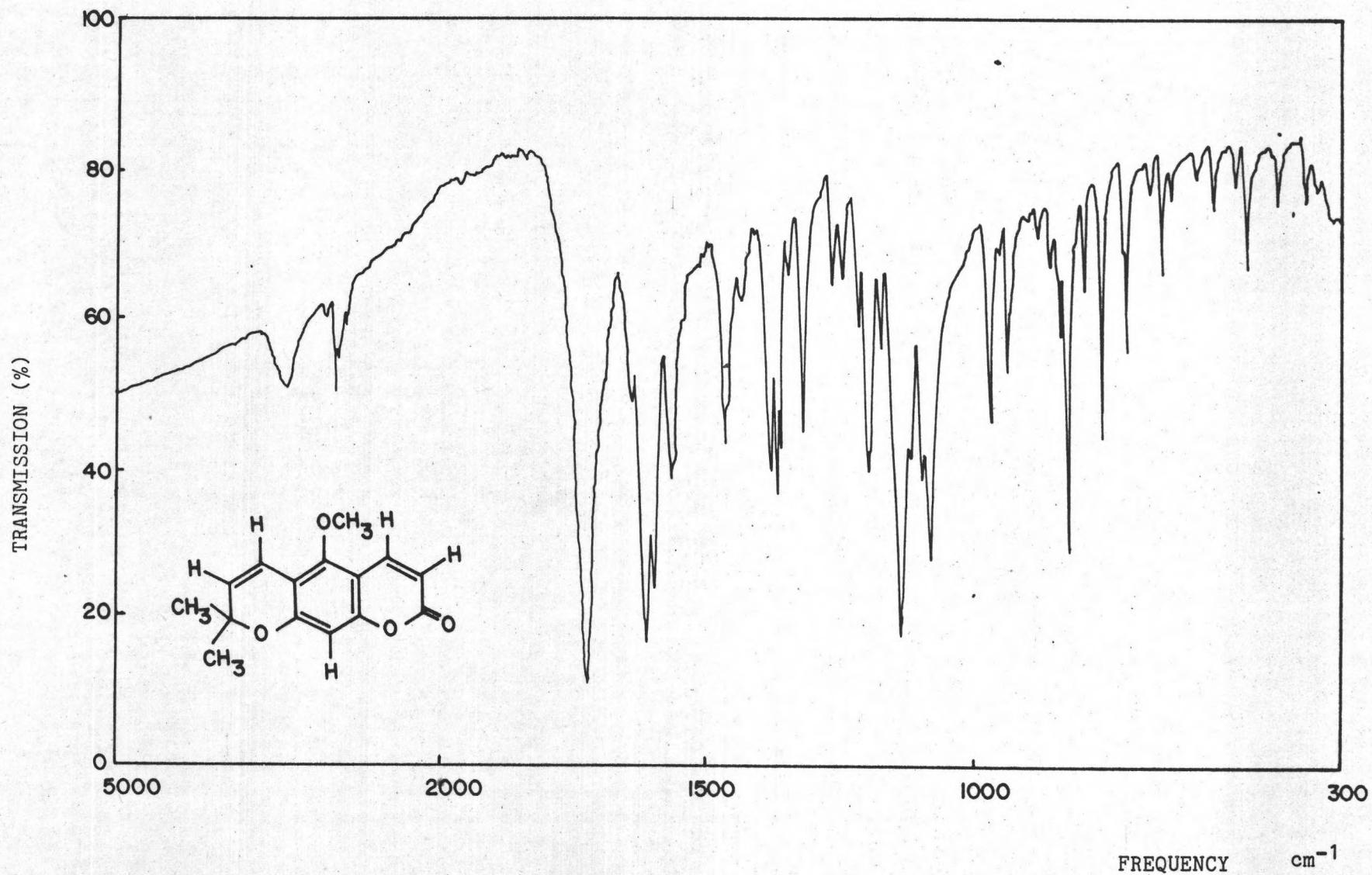
Figure.31 IR spectrum of xanthoxyletin (compound-3)
