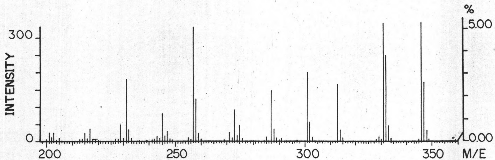
Figure.38 Mass spectrum of compound-4
