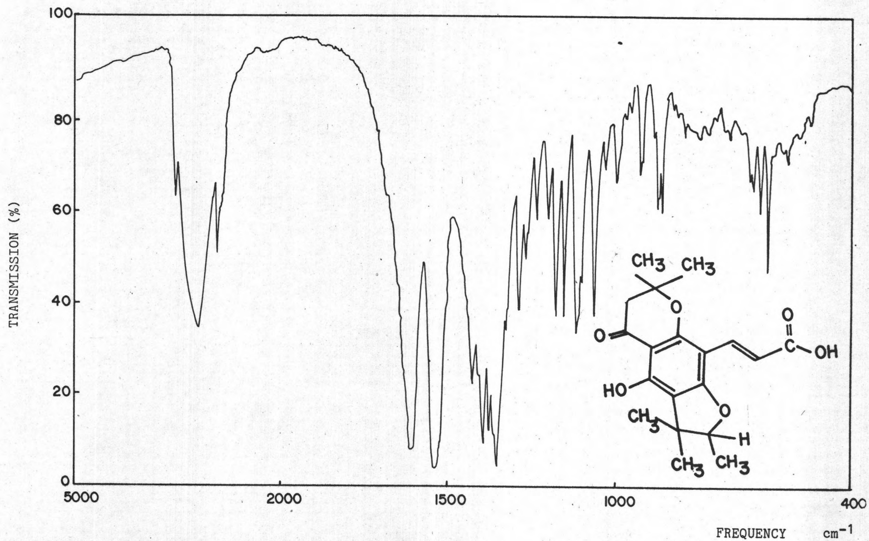
Figure.37 IR-spectrum of compound-4
