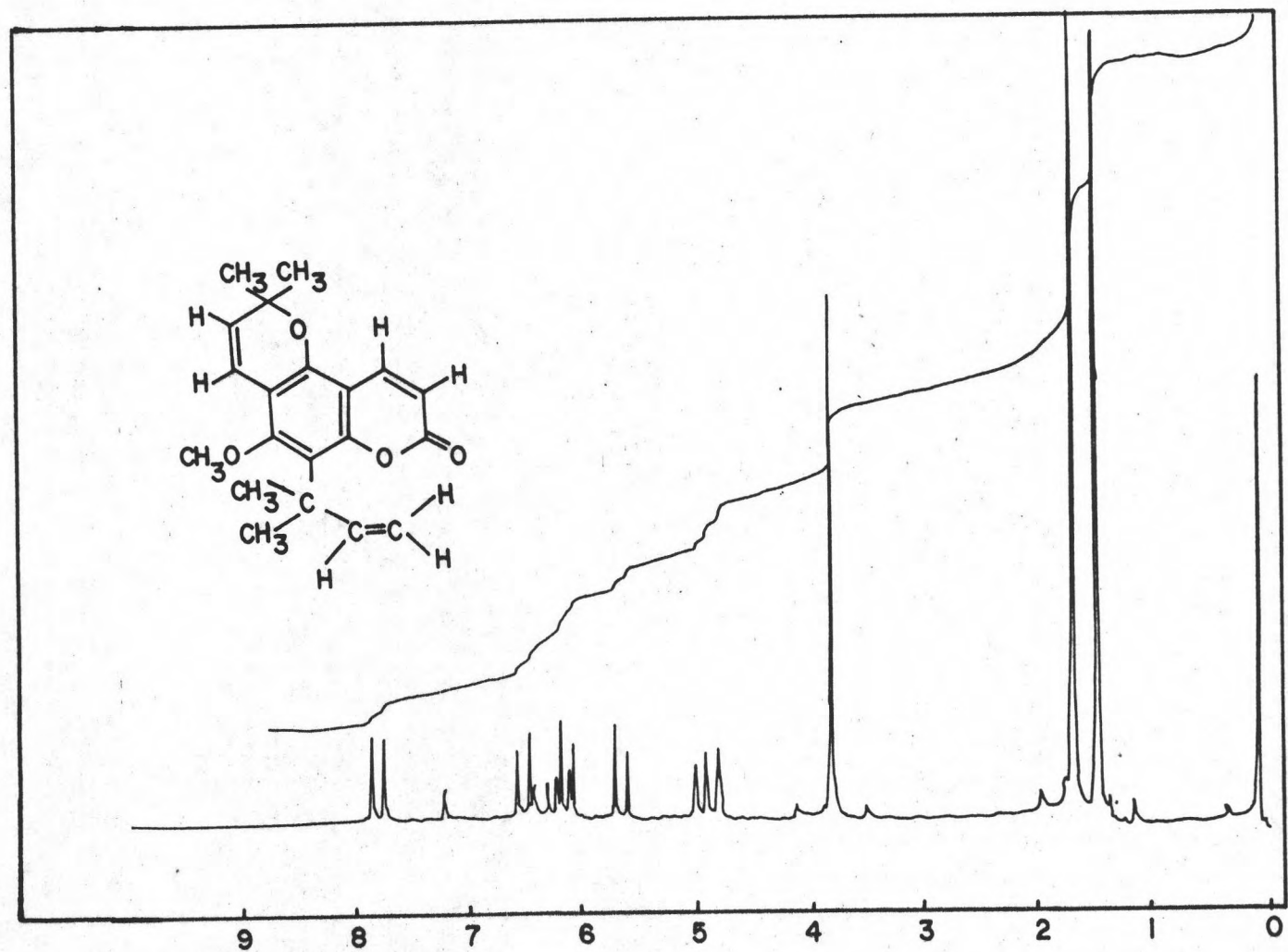
Figure.23 1 H-NMR spectrum of dentatin (compound-1)
