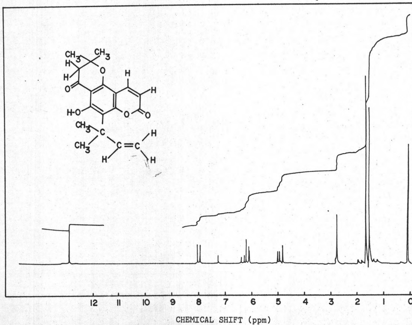
Figure.29 1 H-NMR spectrum of clausenidin (compound-2)
