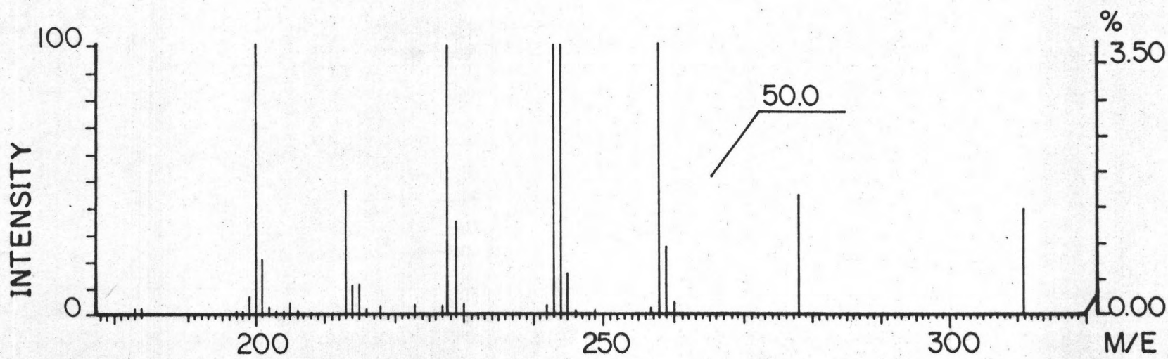
Figure.32 Mass spectrum of xanthoxyletin (compound-3)
