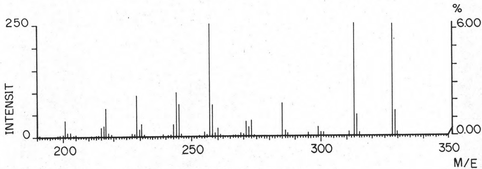
Figure.28 Mass spectrum of clausenidin (compound-2)
