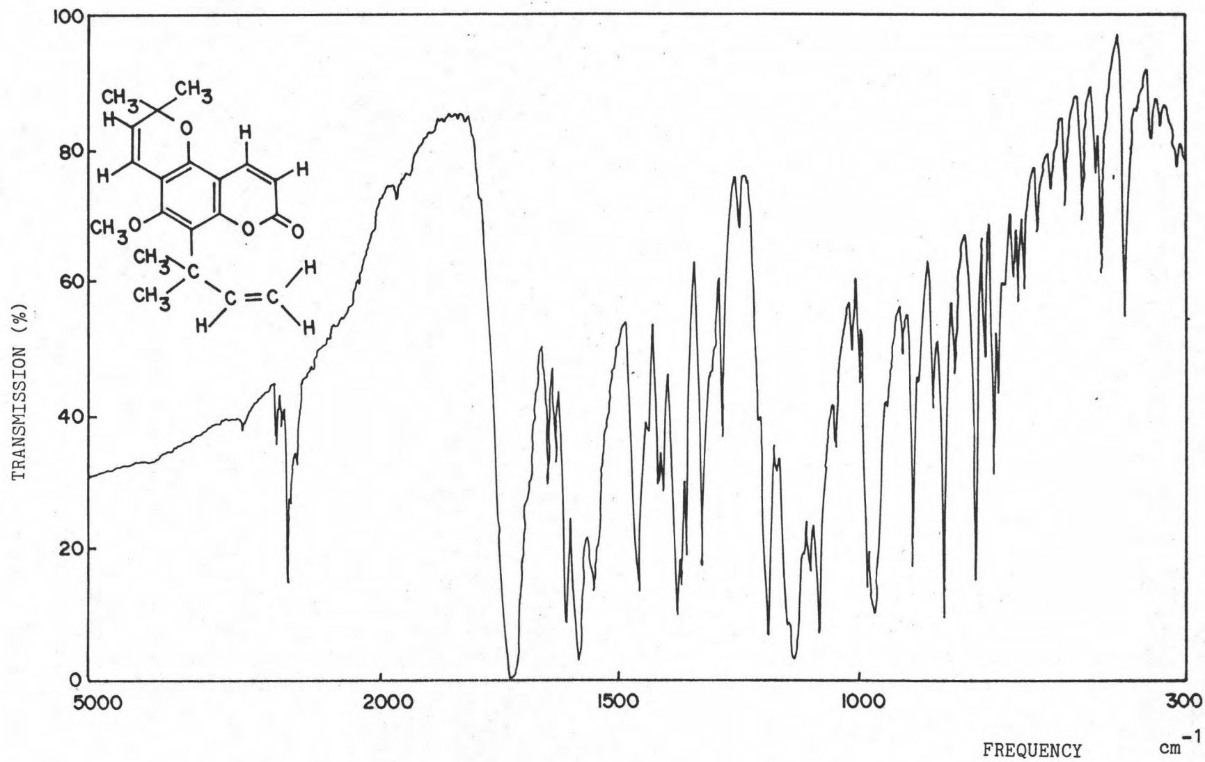
Figure.21 IR spectrum of dentatin(compound-1)
