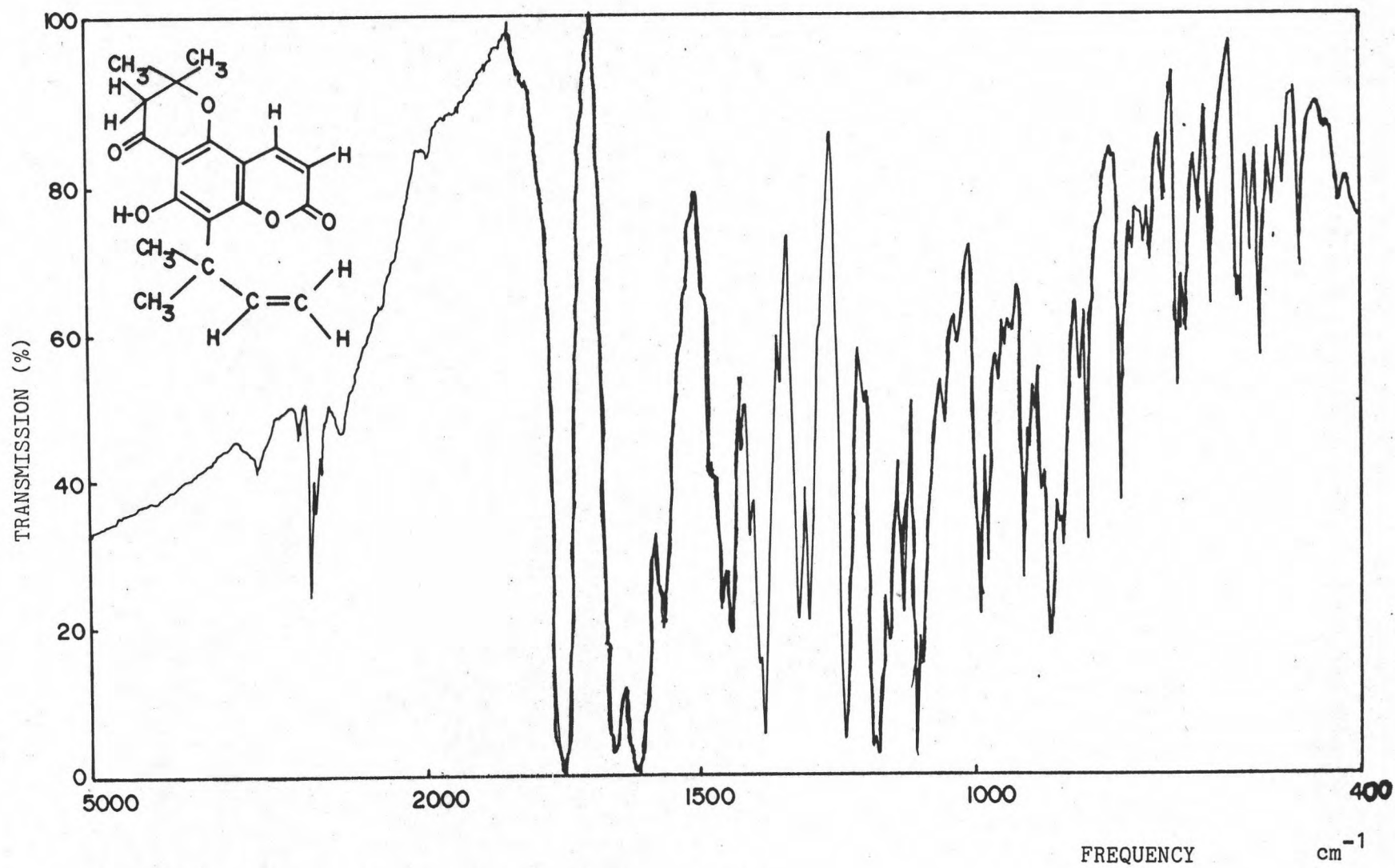
Figure.27 IR spectrum of clausenidin (compound-2)
