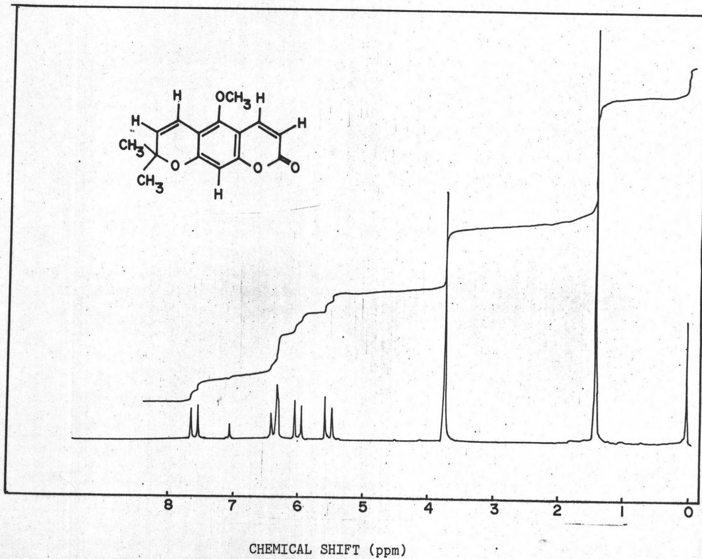
Figure.33 1 H-NMR spectrum of xanthoxyletin (compound-3)
