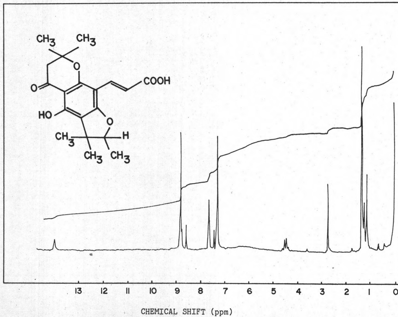
Figure.39 ^1\text{H-NMR} spectrum of compound-4
