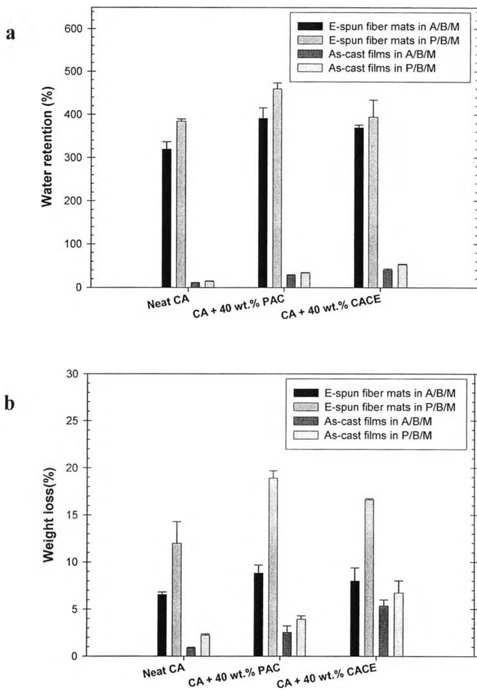
Figure 5.2 (a) Water retention and (b) weight loss behavior of neat, PAC- and CACE-loaded electrospun CA fiber mats and corresponding solvent-cast films in two types of medium, i.e., acetate or phosphate buffer solutions containing 10% v/v methanol ( n = 3 ).
