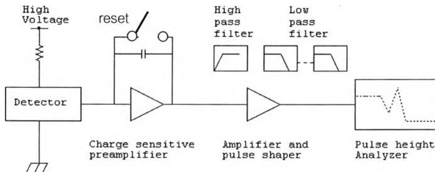
Fig. 1.1 The basic nuclear spectroscopy system
