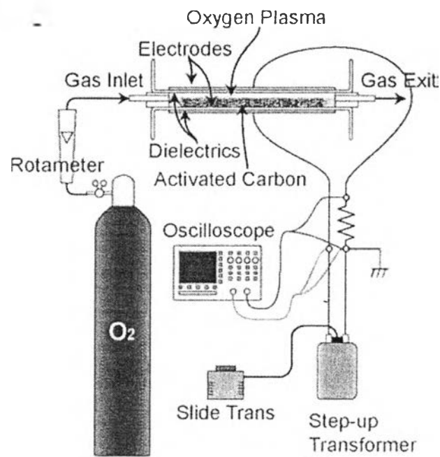
Figure 2.14 Experiment Set up of Dielectric Barrier Discharge Plasma (DBD) (Agostino et al. , 2005).
