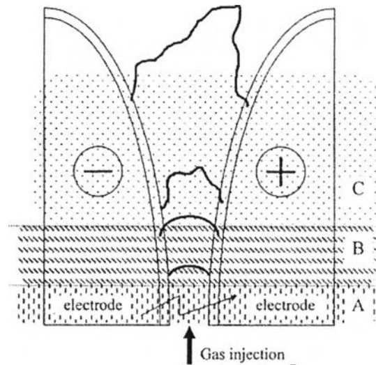
Figure 2.12 Phases of gliding arc evolution: (A) initial gas break-down; (B) equilibrium heating phase; (C) non-equilibrium reaction phase.
