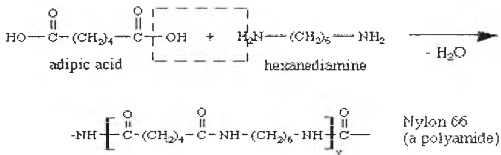
Figure 2.2 Preparation of Nylon 6,6 or Polyamide
