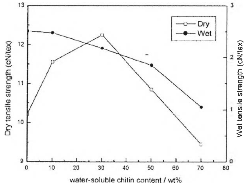
Figure 2.6 The Tendency of Tensile Strength with Chitin Content
