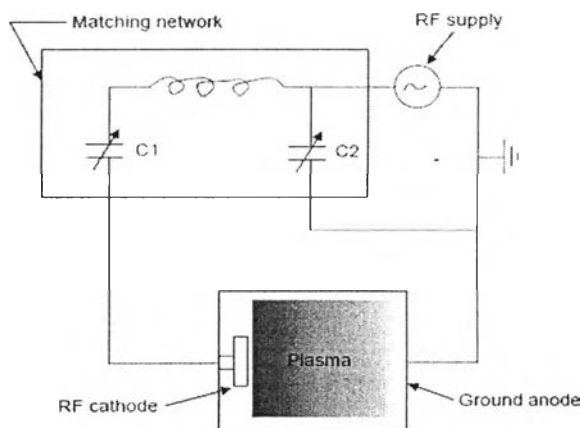
Figure 2.10 Schematic diagram of a capacitively-coupled plasma (CCP) plasma source with an equivalent electrical circuit.
