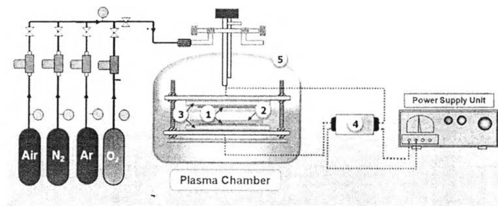
Figure 2.7 Experimental Setup of The DBD system: (1) Electrode Plates (stainless steel plates), (2) Dielectric Plate (glass plate), (3) Acrylic Plates, (4) High Voltage Transformer, and (5) Plasma Chamber
