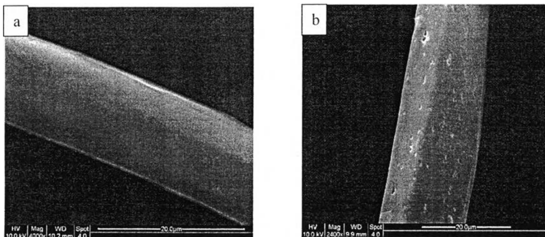
Figure 2.18 SEM images of the Polyester Fibers, (a) Untreated; (b) air/Ar Plasma Treated at a Dielectrics Space of 3 mm for 150 s.
