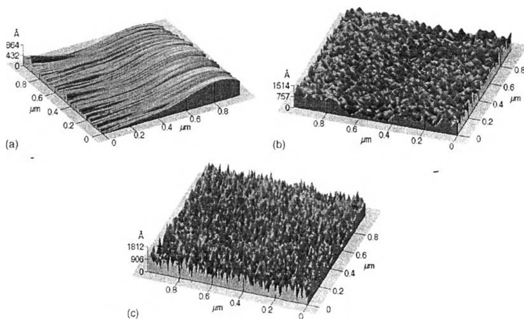
Figure 2.17 3-D views of AFM Images of PET Textile Surface. (a) Untreated Surface; (b) 60 s Treated Surface; (c) 120 s Treated Surface
