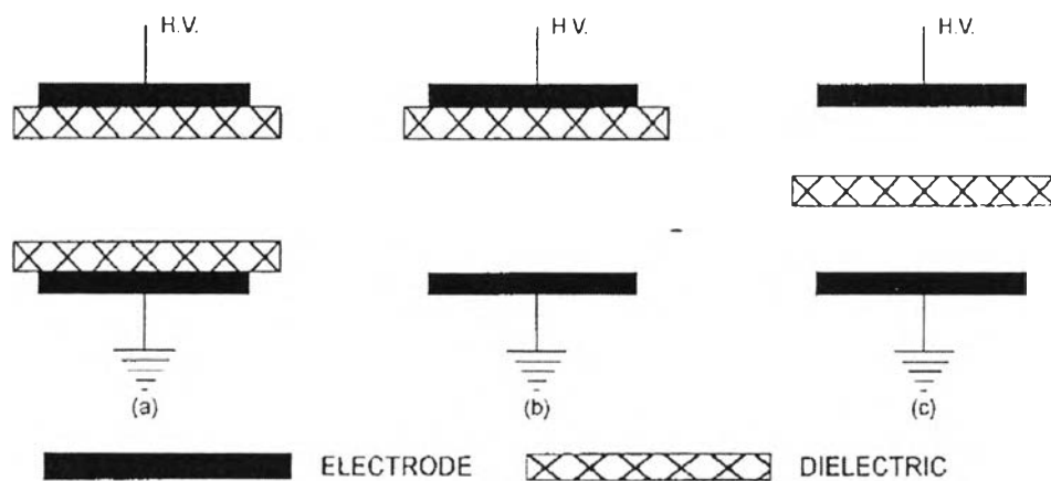
Figure 2.15 Schematic Diagram of Parallel-Plate DBD Plasma Source Configurations.
