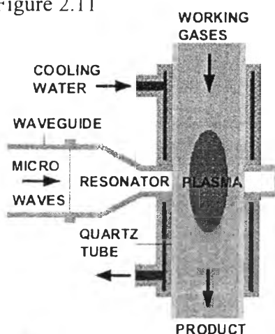
Figure 2.11 Schematic drawing of Microwave discharge.
