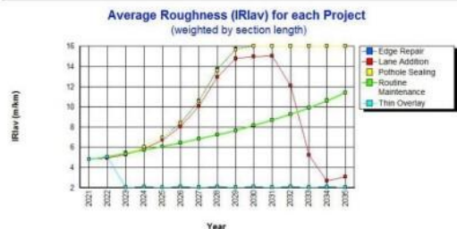
HDM - 4 Average Roughness by Project (Graph) Study Name: Rural roads (SS3) Run Date: 02-03-2021
