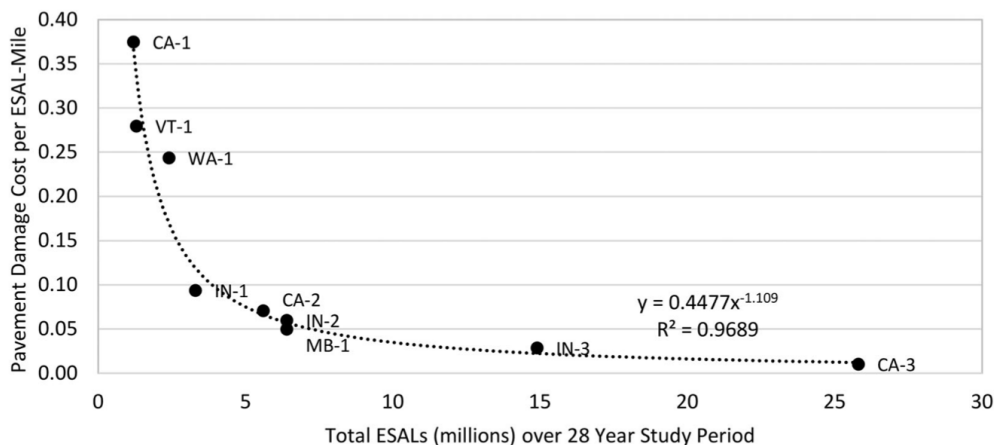
Relationship between Pavement Damage Cost per ESAL-Mile and Loading (ESALs) for Sections with Strength of 6 to 8 SN.
