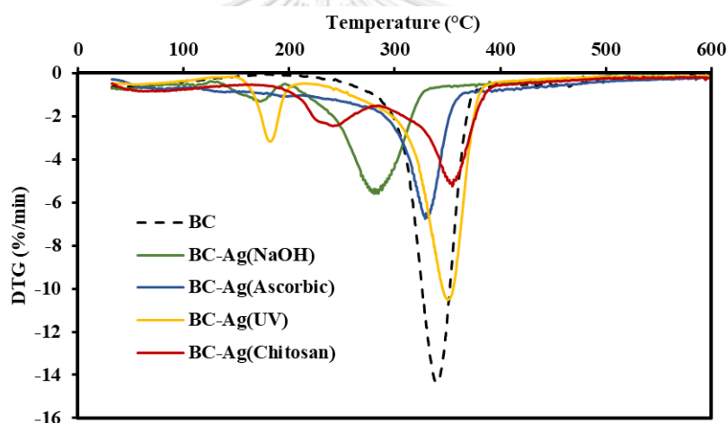
Figure 14. DTG curves of BC and BC-Ag composites.
